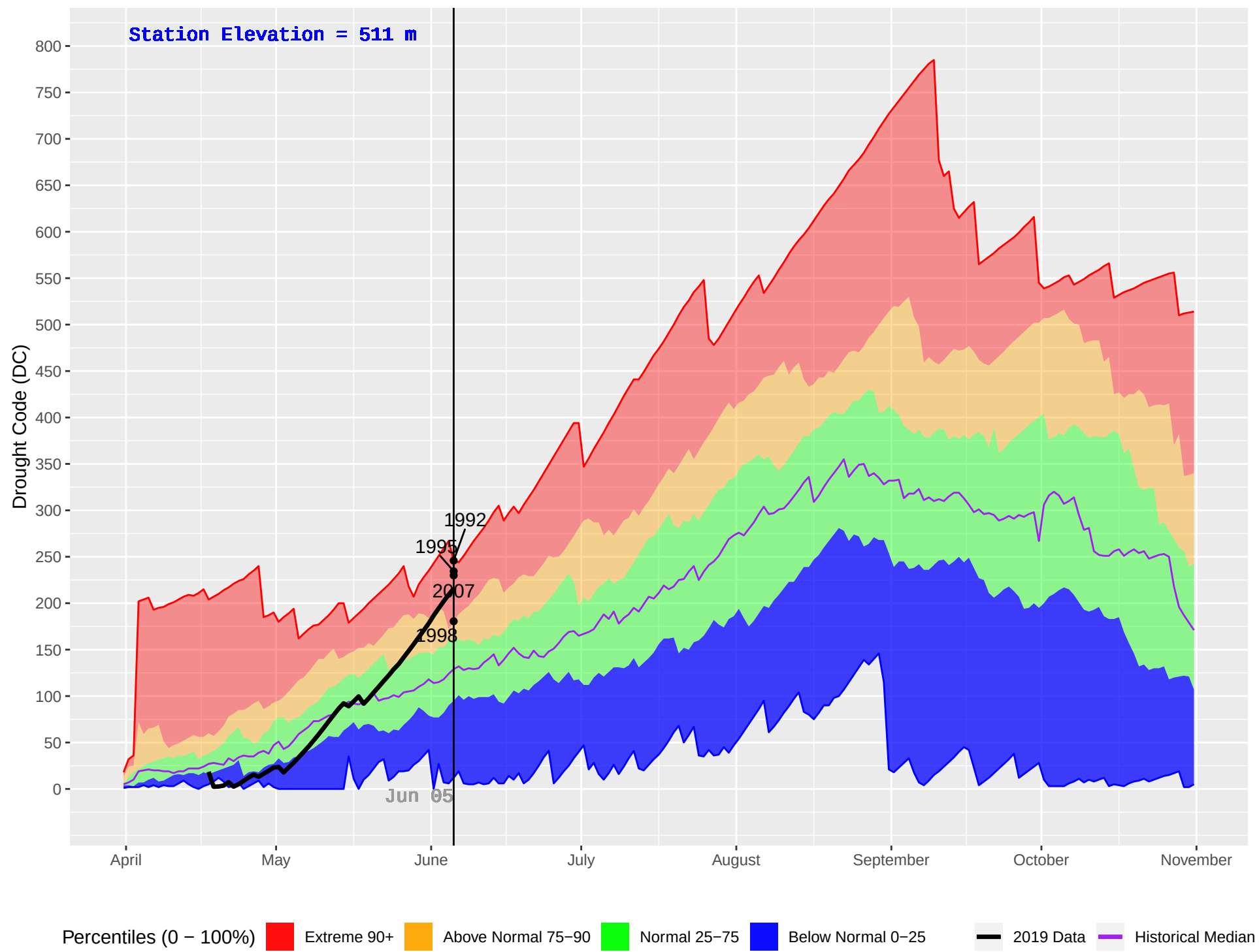
SEYMOUR ARM (344) : Historical (1981–2018) and Current (2019) Daily Drought Code (DC)
