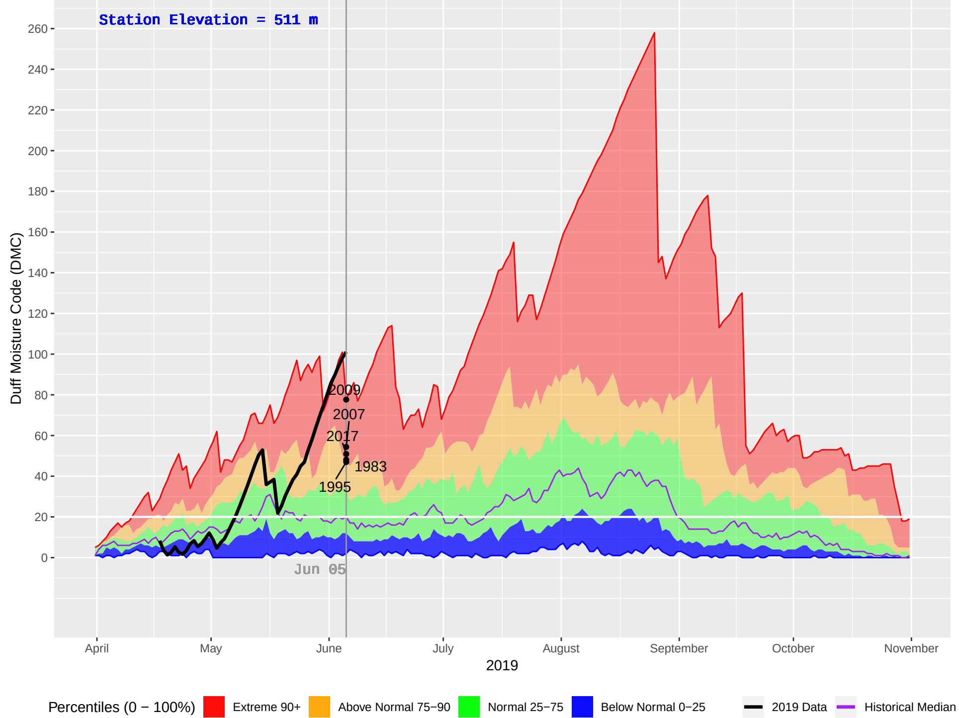
SEYMOUR ARM (344) : Historical (1981–2018), Current (2019) Daily Duff Moisture Code (DMC)
