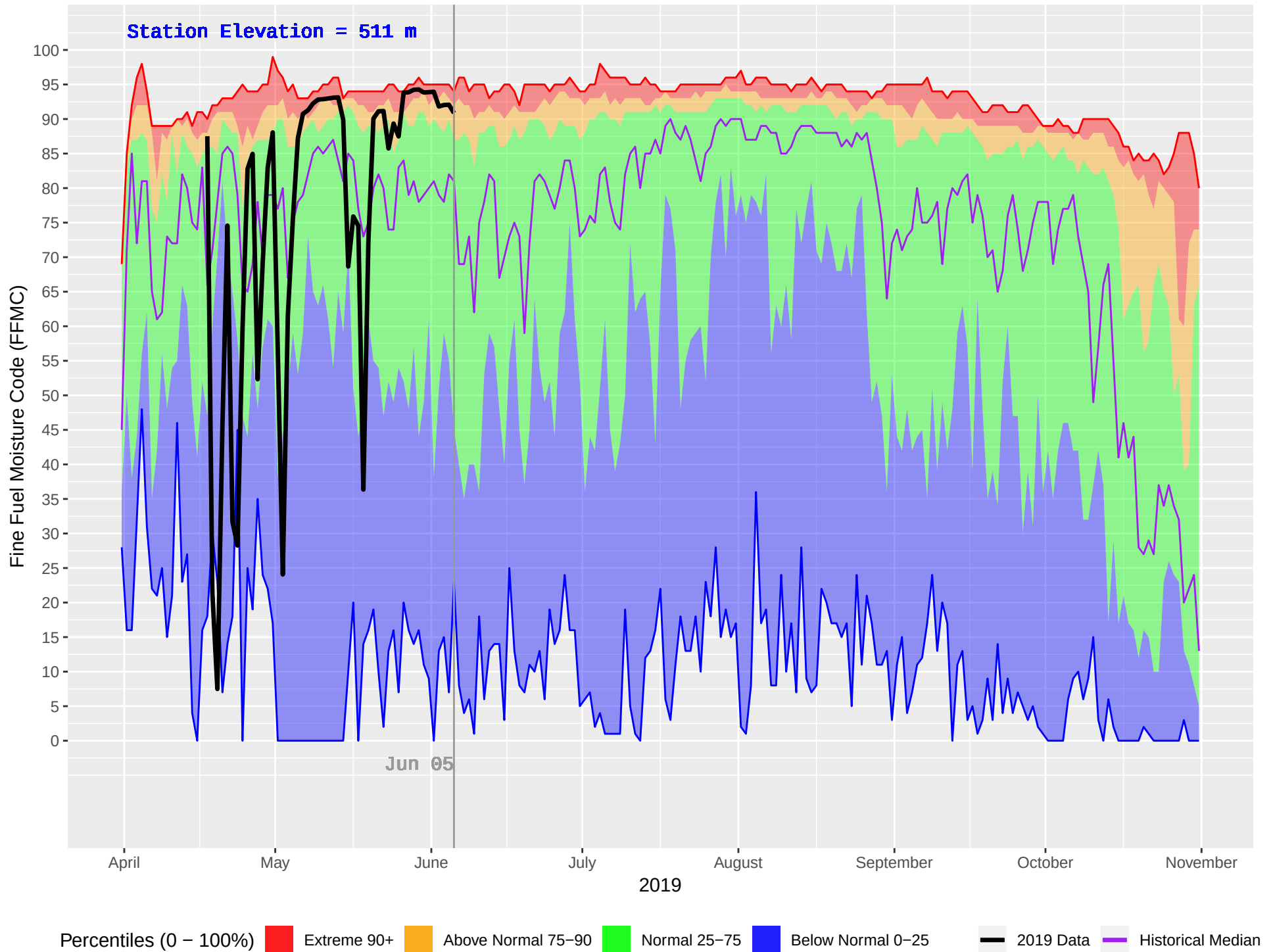
SEYMOUR ARM (344) : Historical (1981–2018) and Current (2019) Daily Fine Fuel Moisture Code (FFMC)
