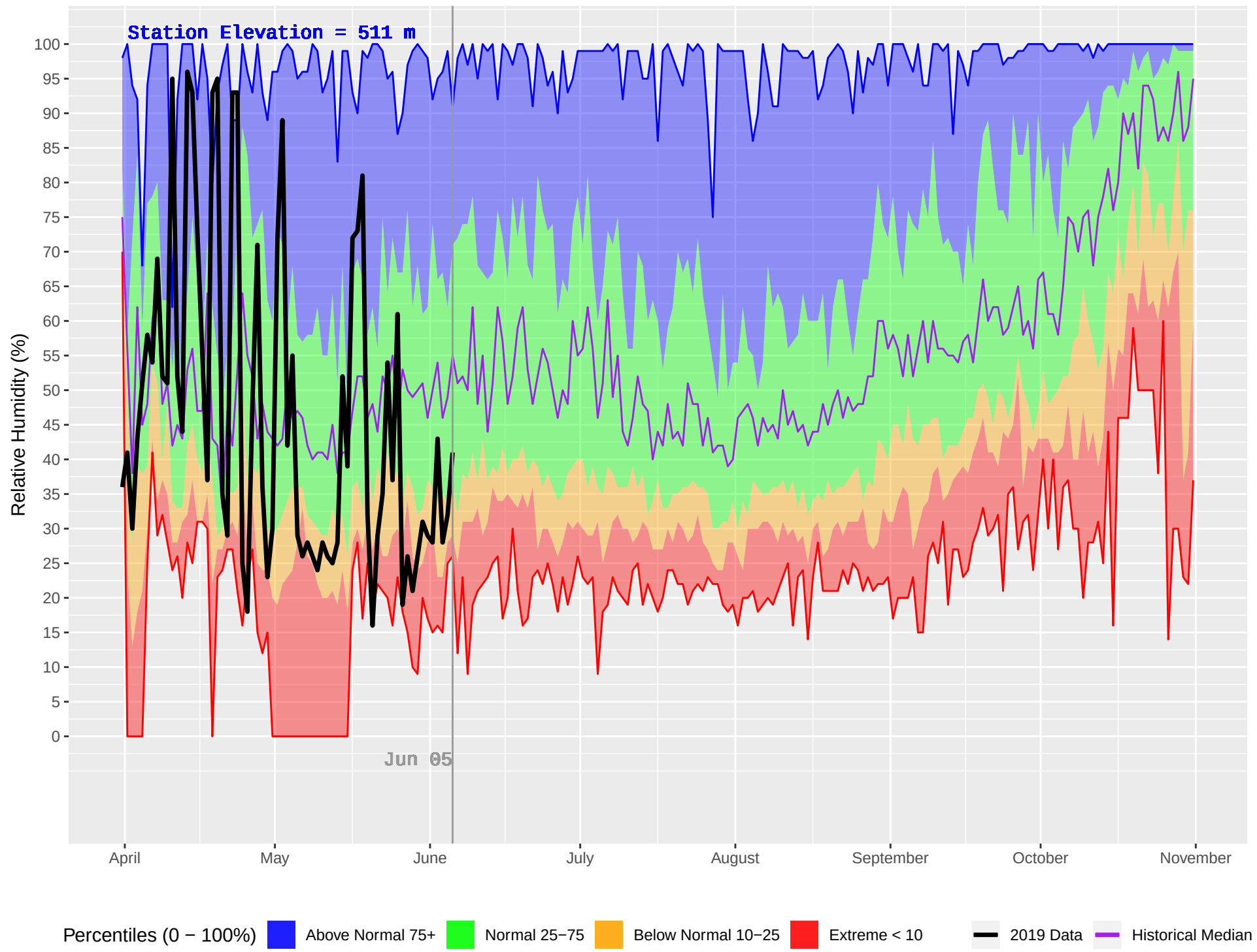
SEYMOUR ARM (344) : Historical (1981–2018) and Current (2019) Daily Relative Humidity
