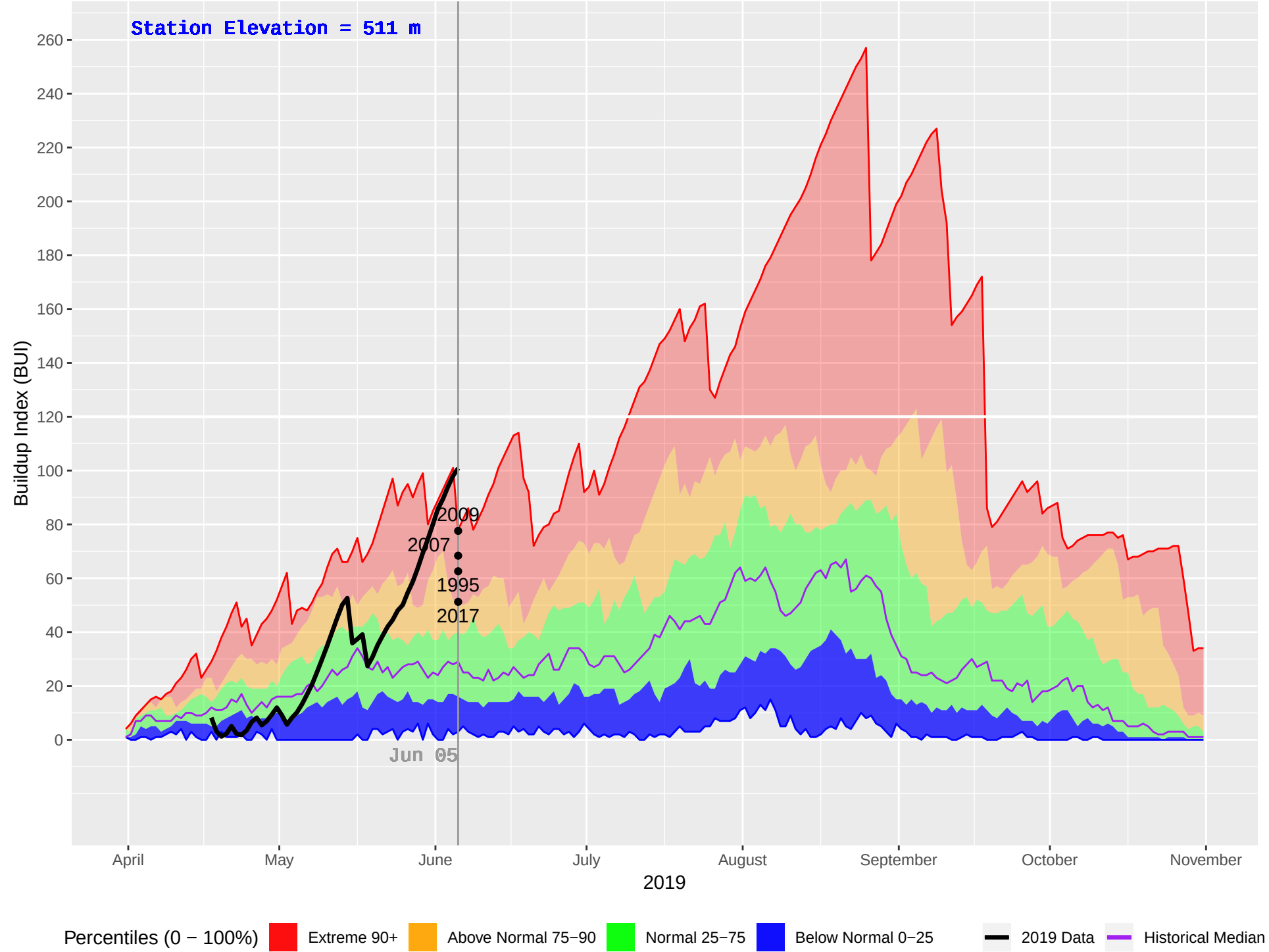
SEYMOUR ARM (344) : Historical (1981–2018), Current (2019) Daily Buildup Index (BUI)
